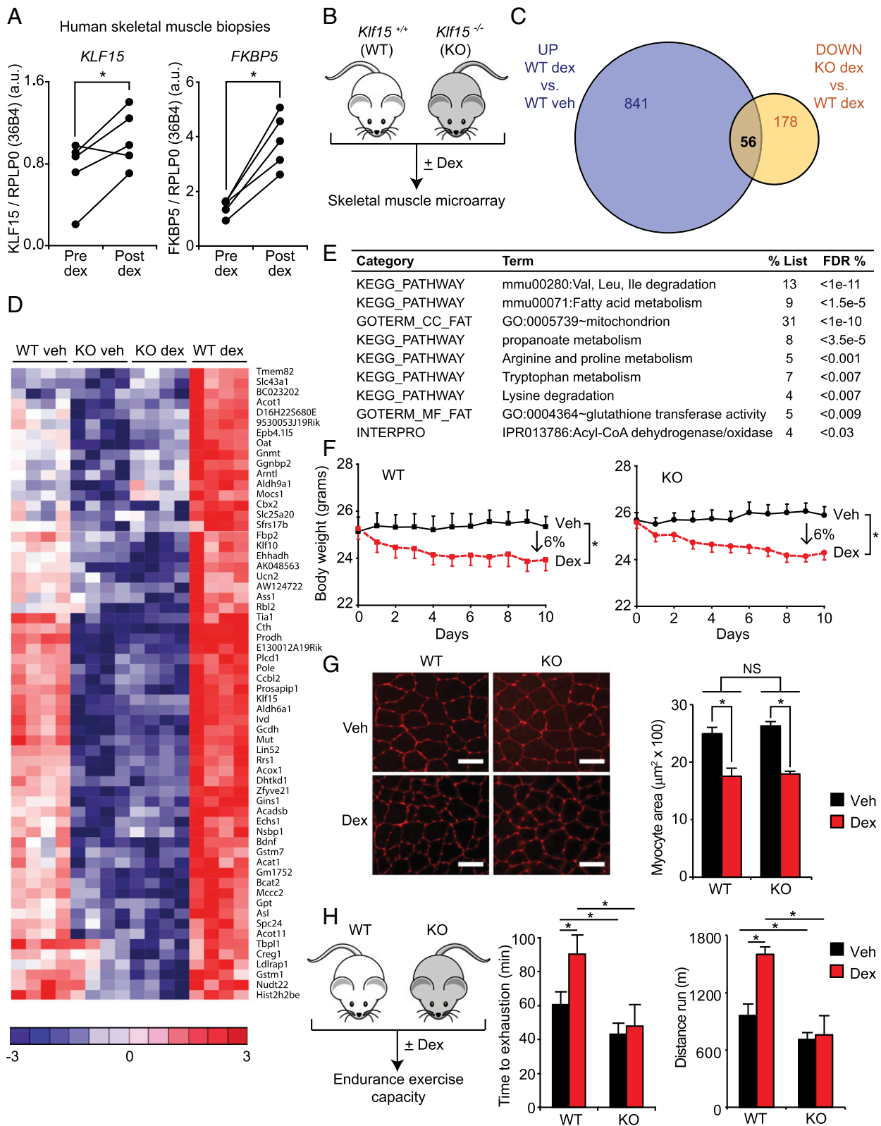
Fig. 1. The GC-KLF15 axis dissociates ergogenic physiology from muscle atrophy. (A) KLF15 expression in skeletal muscle of healthy human subjects pre- and post-dex administration. FKBP5 is a known direct GR target shown as a positive control ( n = 5 ; *P < 0.05 for indicated comparisons). (B) Schematic for skeletal muscle (quadriceps) microarray study ( n = 4 per group). (C) Venn diagram of dex-inducible and KLF15 -regulated genes [2 mg/kg i.p. \times 1 dose, 8 h time point; fold change > 1.5 and false discovery rate (FDR) < 0.05 ]. (D) Heat map of genes robustly regulated [family-wise error rate (FWER) < 0.05 ] by GC-KLF15 axis in mouse skeletal muscle. (E) Functional annotation [Database for Annotation, Visualization, and Integrated Discovery (DAVID)] of genes regulated by GC-KLF15 axis. (F) Body weight and (G) muscle (tibialis anterior) histology [wheat-germ agglutinin (WGA) stain] and cross-sectional area in a mouse model of chronic dex-induced atrophy (1 mg/kg d.s.c. \times 10 d; n = 8 ; *P < 0.05 for indicated comparisons). (Scale bar, 50 \mu\text{m} .) (H) Schematic of dex-induced doping experiment (2 mg/kg i.p. \times 1 dose) with time to exhaustion and distance run on a motorized treadmill 18 h post-dex administration ( n = 7-9 ; *P < 0.05 for indicated comparisons). Data are shown as mean \pm SEM.
